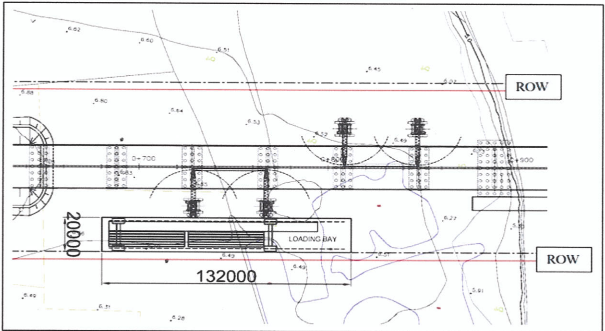
Enlarged View of Right Bank Side Construction Yards
