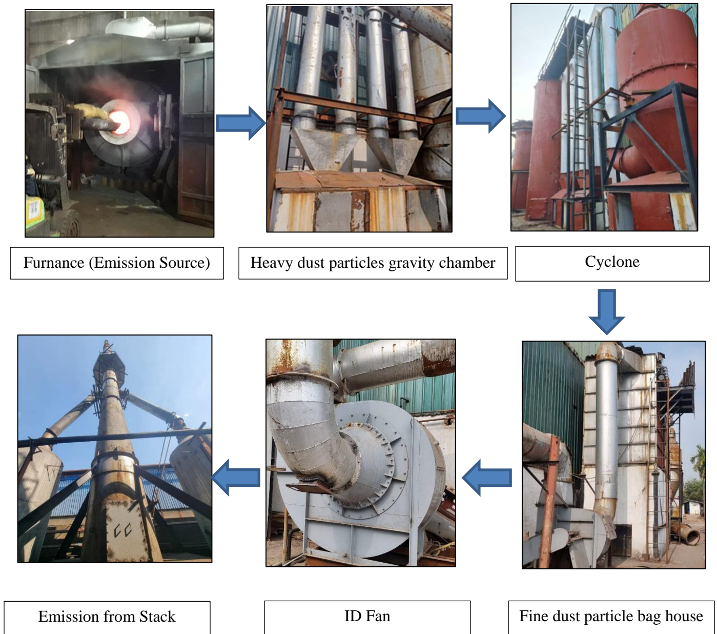
Figure 7.4 Photos of Air Pollutants Control System
