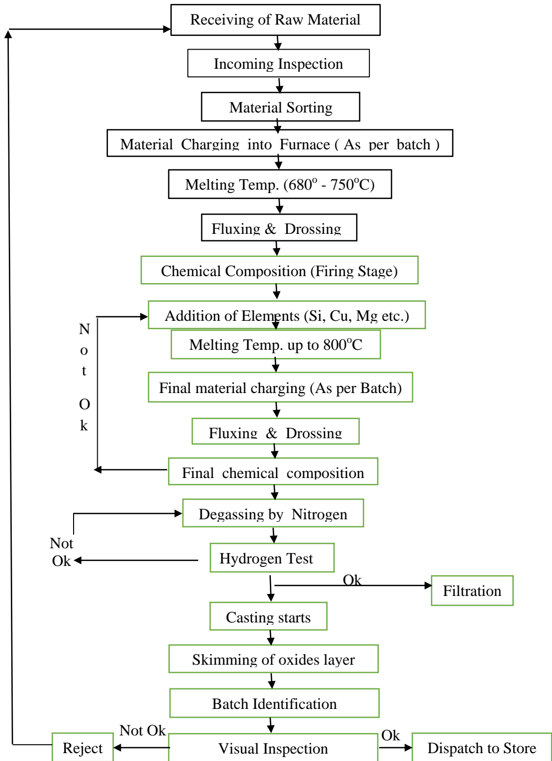
Figure 3.41 MYSARCO’s Process Flow Chart for Manufacturing of Aluminum Ingot
