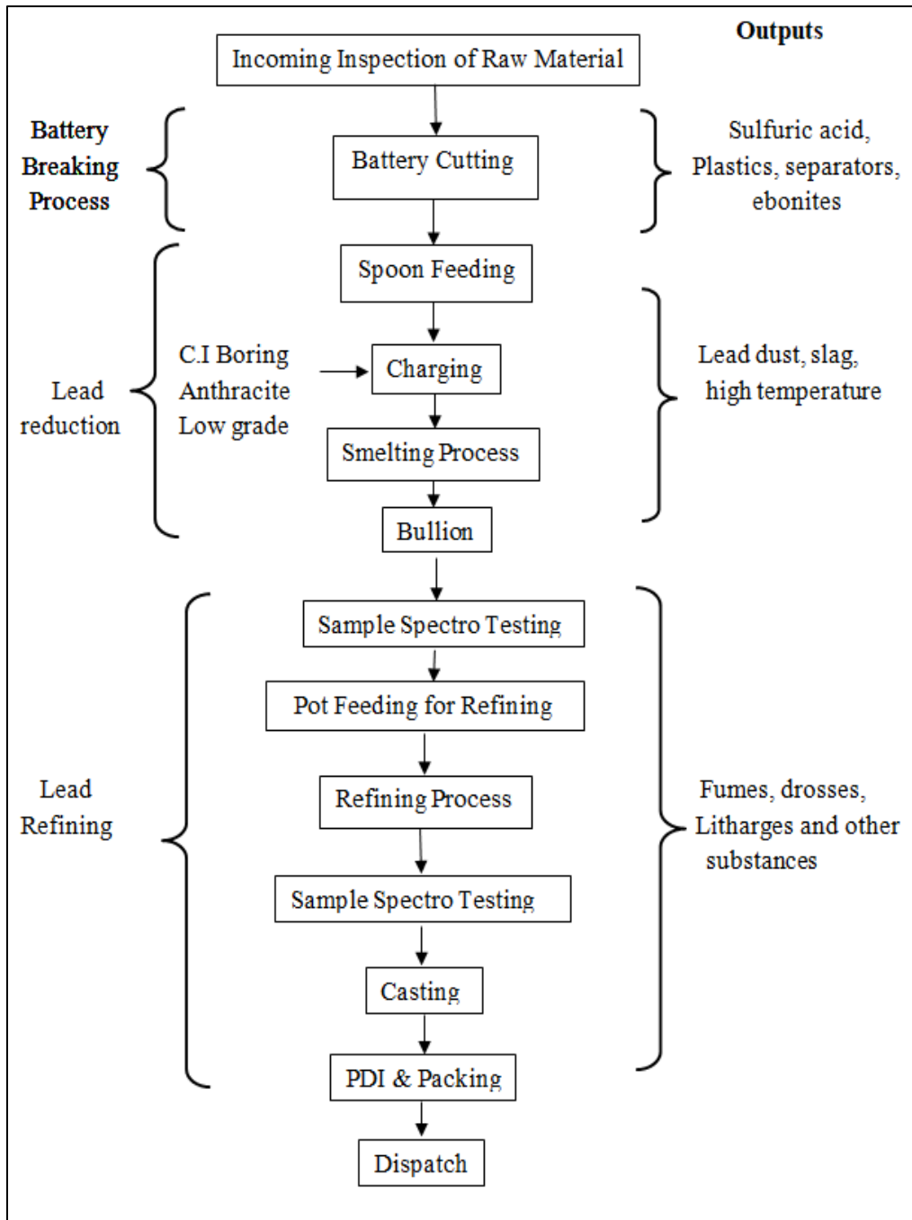
Figure 3.30 MYSARCO’s Process Flow Chart for Manufacturing of Lead/Lead Alloy
