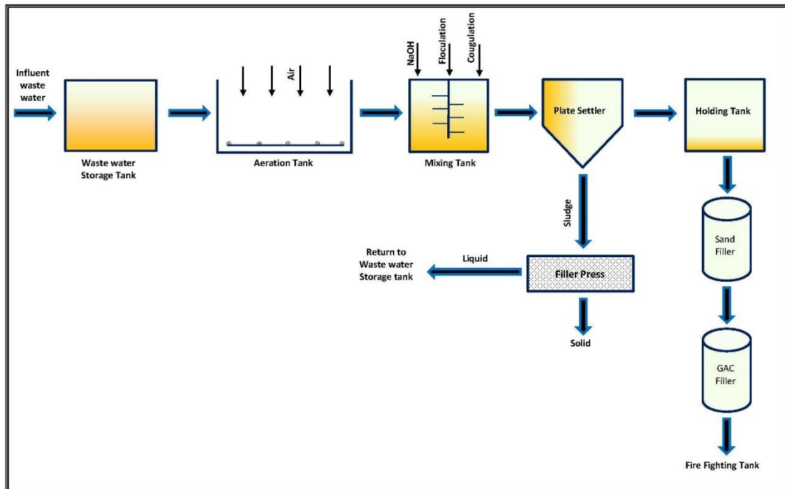
Figure 7.8 Wastewater Treatment Plant
