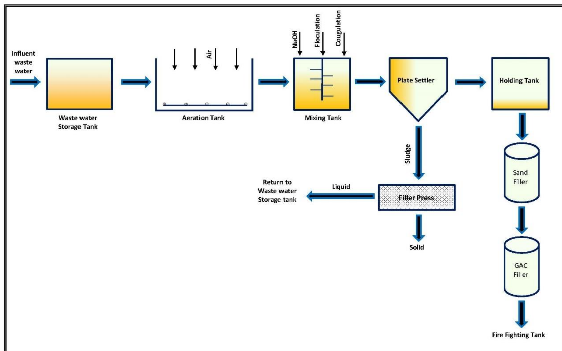
Figure 3.16 Wastewater Treatment Plant
