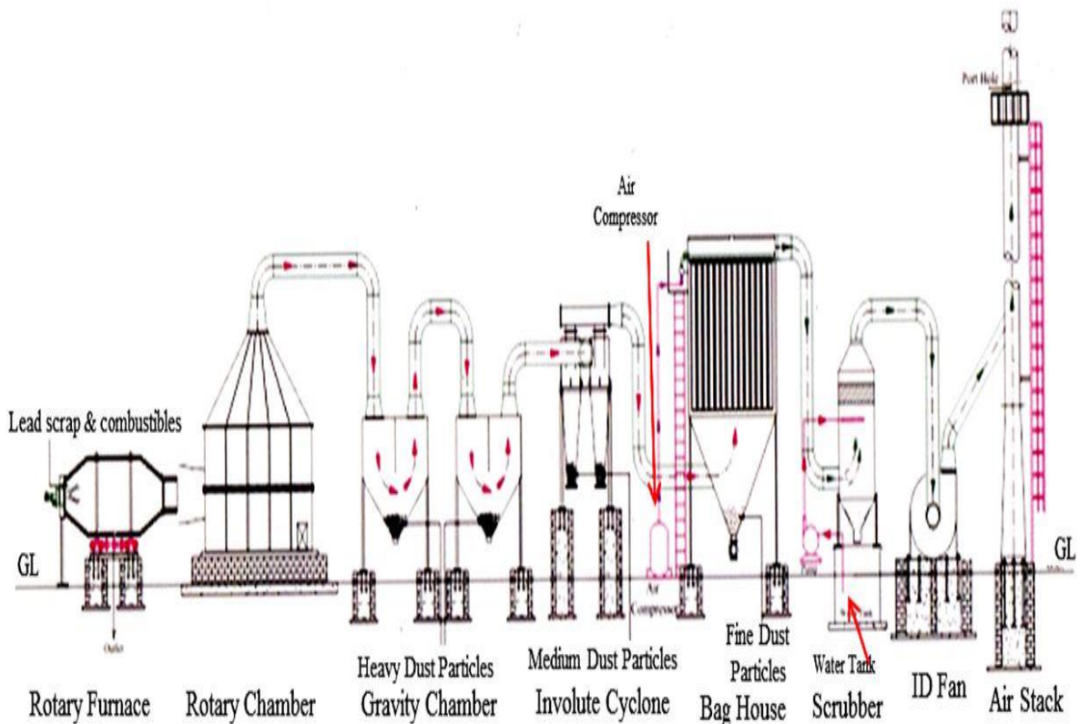
Figure 6 Rotary Furnaces with Complete Pollution Control Equipment
