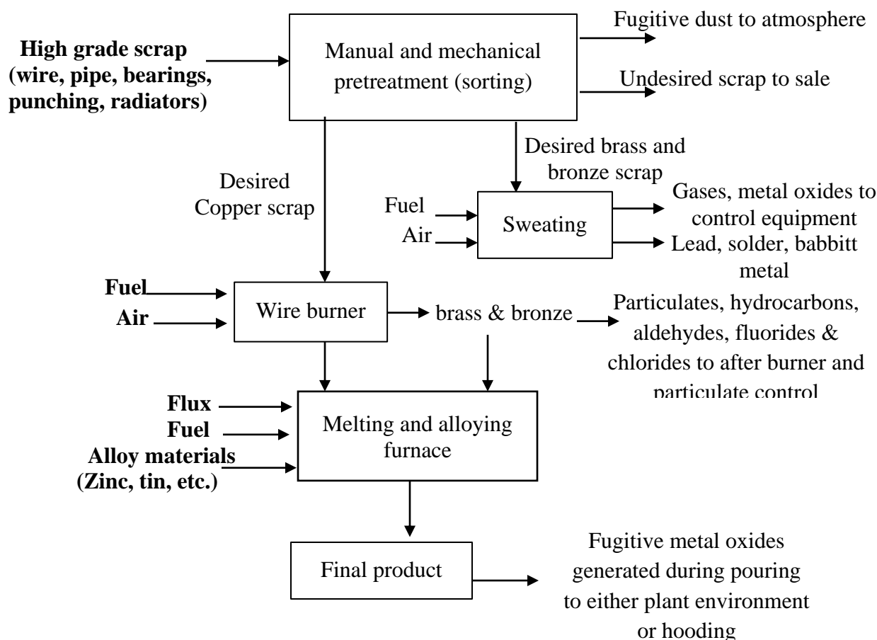
Figure 3.43 High Grade Brass and Bronze Alloying Production Process
