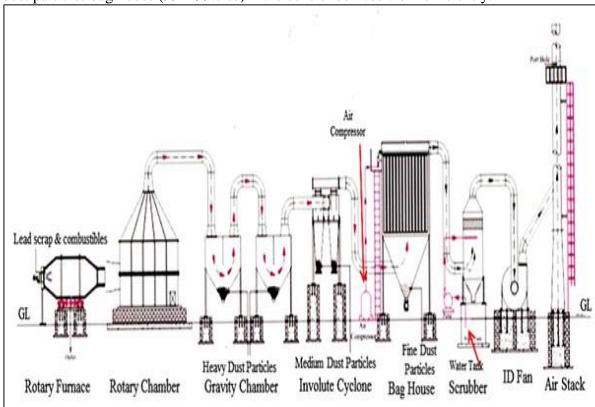
Figure 7.3 Air Pollutants Control System
