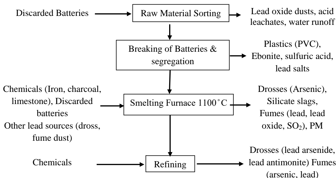
Figure 5.1 Input and Output streams from Smelting and Refining of Used Batteries
