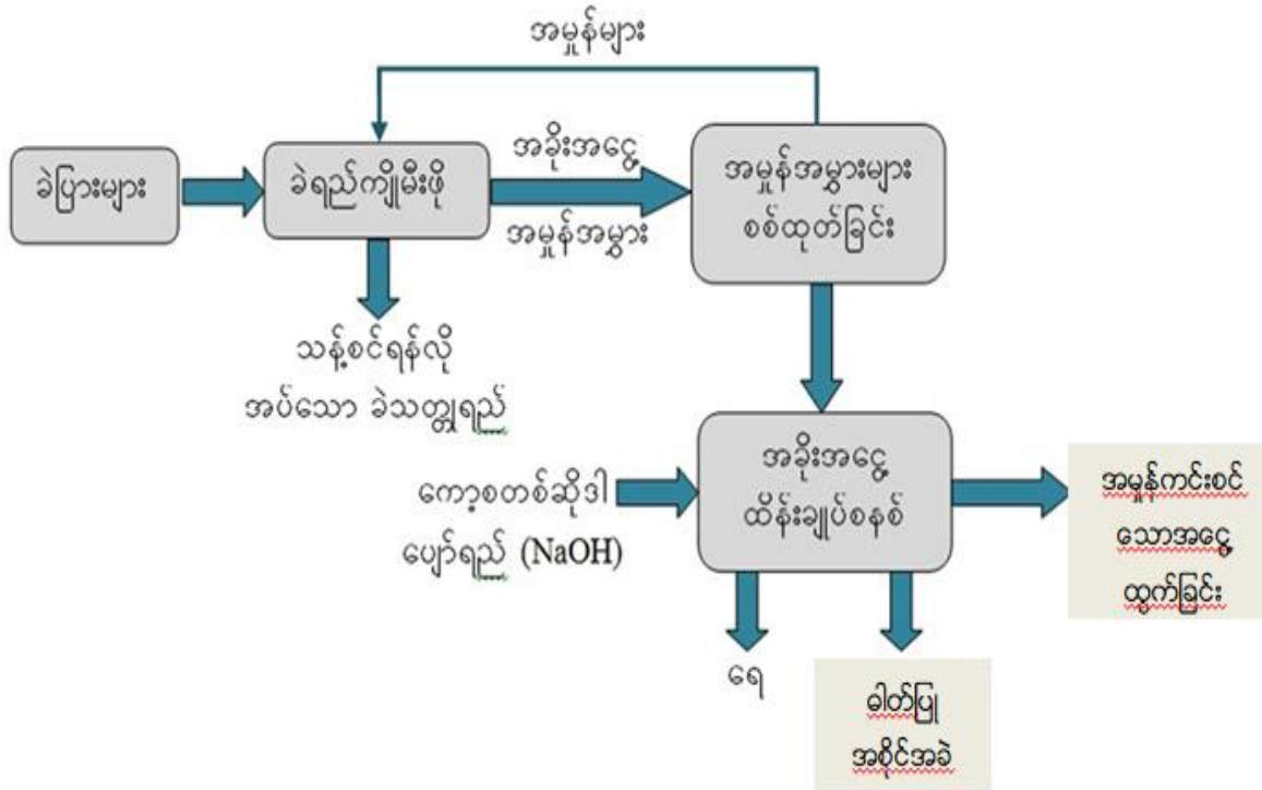
Figure 5 Pollution Control System for Lead Smelting Furnace
