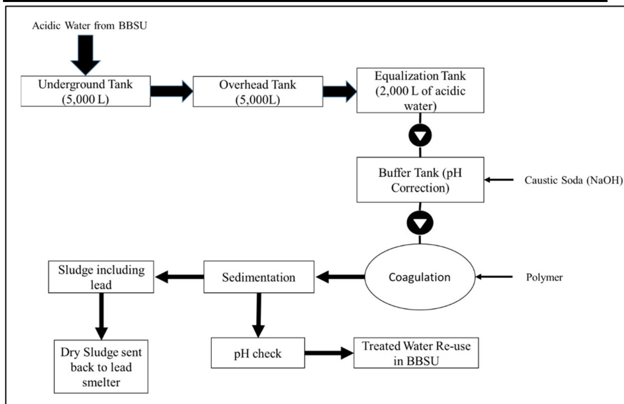
Figure 3.31 Acidic Wastewater Treatment System Flow Diagram
