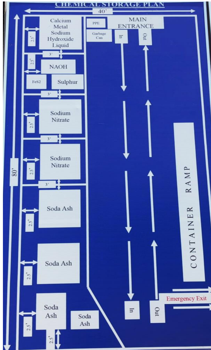
Figure 3.26 Layout Plan of Chemicals Storage Area
