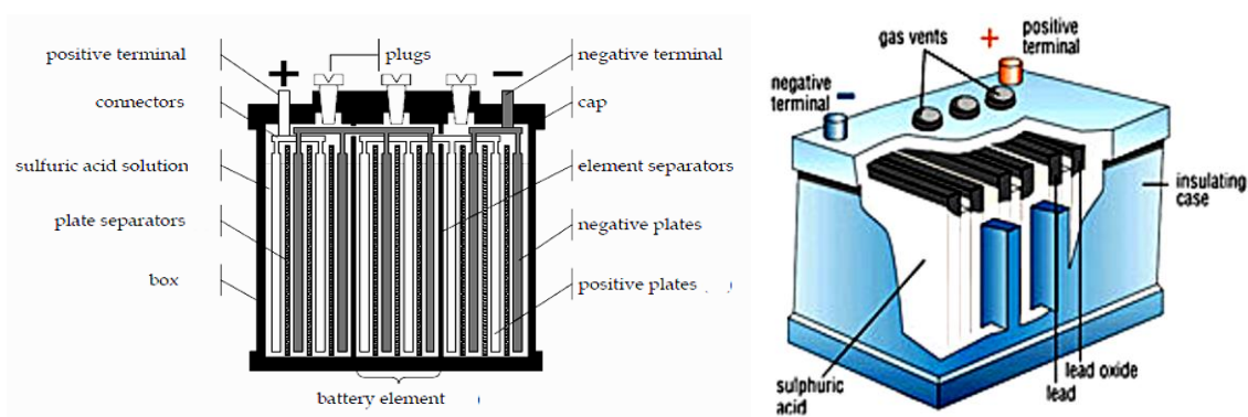
Figure 3.22 Lead-Acid Battery Components and Internal Structure
