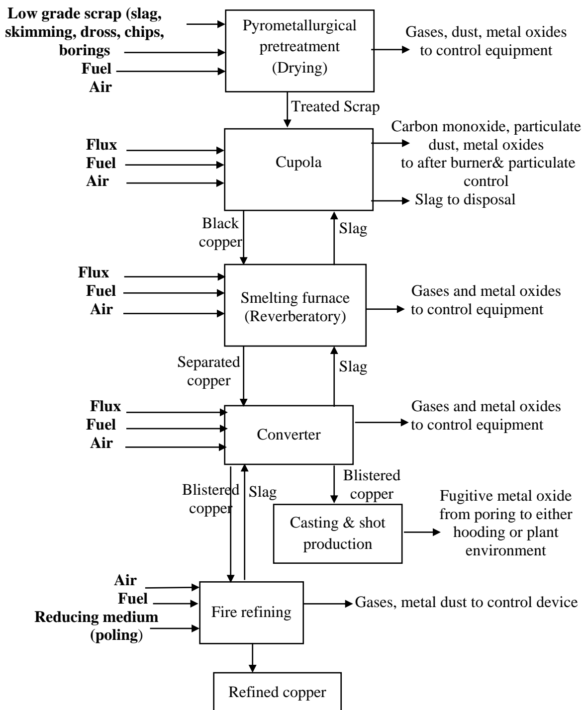
Figure 3.42 Low Grade Copper Recovery Process Flow Diagram
