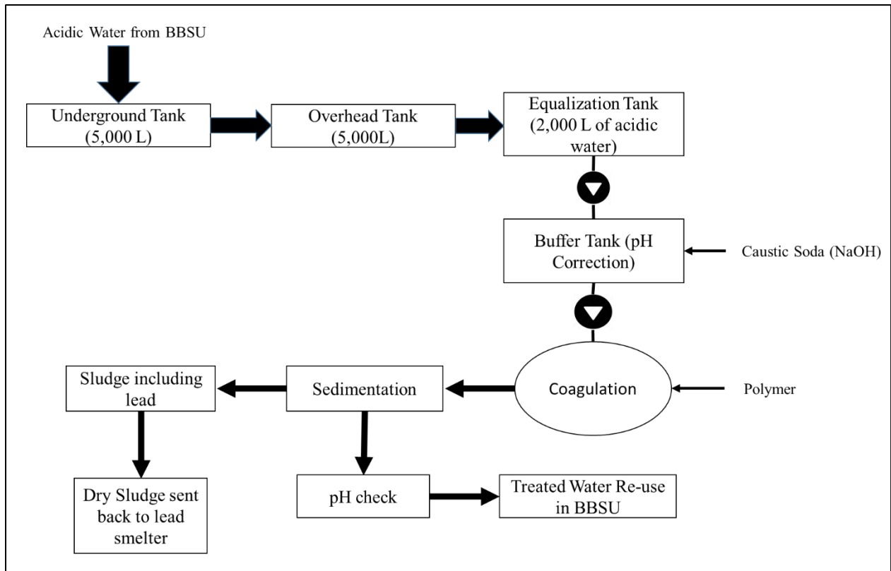
Figure 7.7 Effluent Treatment System
