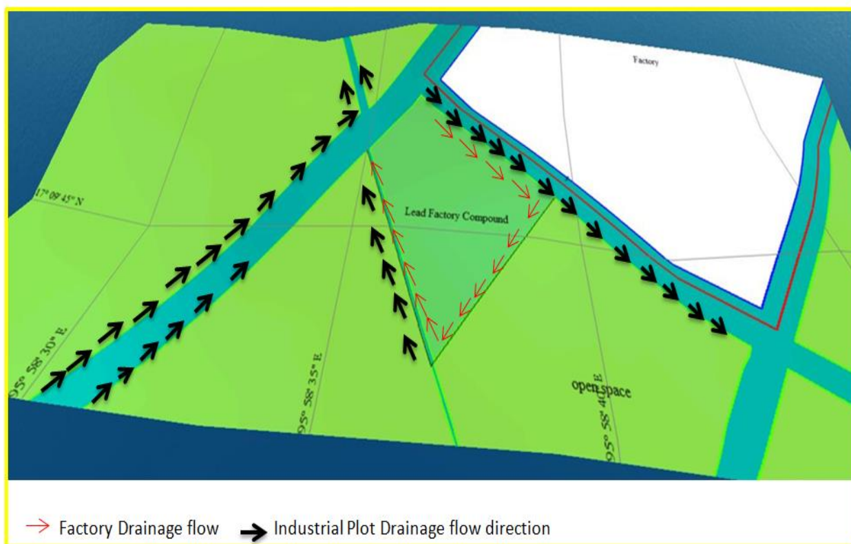
Figure 4.8 Flow Direction of Factory and Road Drainage Flow Direction
