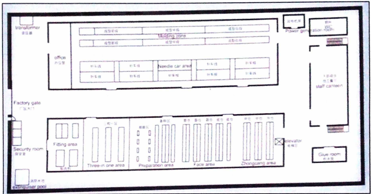
Figure 0-5: Floor Plan of Factory
